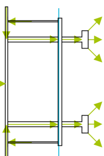
wall detail [1:20]
